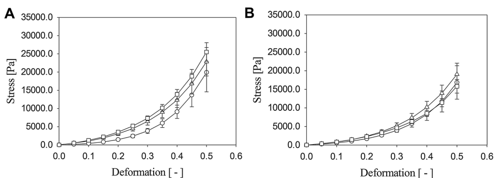
Fig. 4. Mechanical strength of alginate beads. (A) effect of alginate concentration at constant calcium concentration of 0.1 M \text{CaCl}_2 : ( \circ ) 1.2% (w/v) alginate, ( \Delta ) 1.8% (w/v) alginate, ( \square ) 2.4% (w/v); (B) effect of calcium concentration at constant alginate concentration 1.2% (w/v) alginate: ( \circ ) 0.07 M \text{CaCl}_2 , ( \Delta ) 0.1 M \text{CaCl}_2 , ( \square ) 0.15 M \text{CaCl}_2 .
