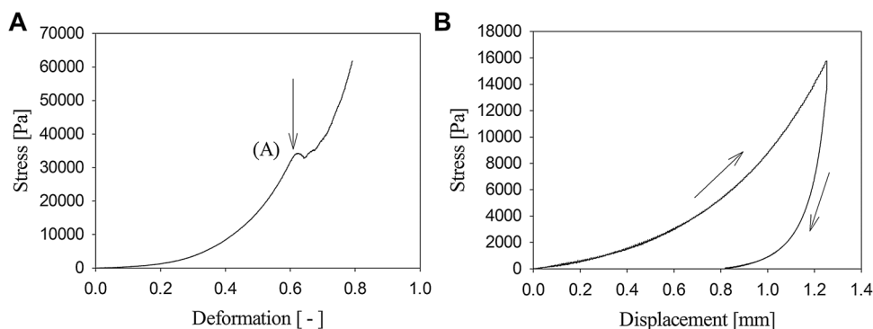
Fig. 3. Mechanical properties of calcium alginate beads. (A) stress as a function of deformation, (B) example of press-release curve in 1.2% (w/v) alginate gelled in and 100 mM \text{CaCl}_2 .
